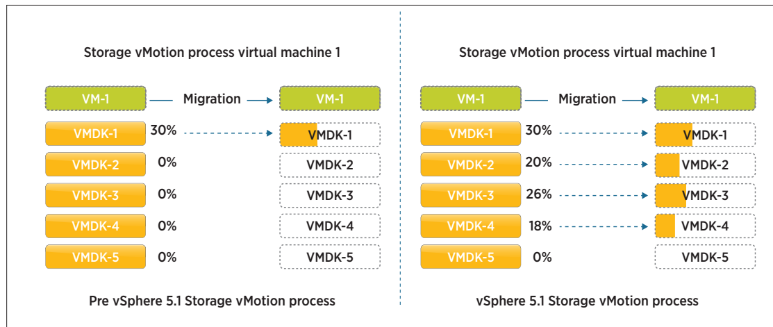
Figure 7. Storage vMotion
